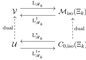
Figure 1. Relationships between the function spaces.
